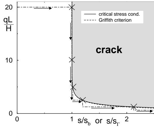
FIG. 3. The shrinking rate at the first breaking under the fixed boundary condition is plotted as a function of the system size, where the vertical axis represents qL scaled by H and the horizontal axis is s scaled by s_b or s_r . The dotted line represents the result for the Griffith criterion.
